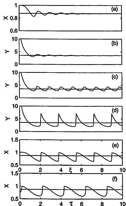
Figure 2. Steady-state profiles of the dimensionless concentration ( x ) (a, e) and temperature ( y ) for Pe = 14 (a, b), 20 (c), 100 (d, e) of the full system (3) and the corresponding CSTR dynamic behavior (f).
